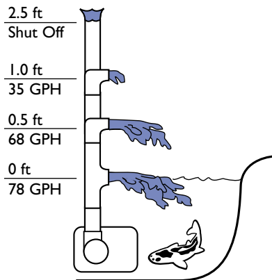
DP80 Pump Flow Chart Average Performance gph = gallons per hour
